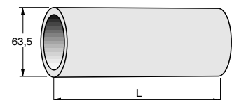
3 Mounting Tube: Length 305 mm - Part no. 43791-12 Length 457mm - Part no. 43791-18 Length 610 mm - Part no. 43791-24
