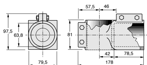
4 Tee Mount - Part no. 43790
