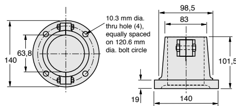
1 Base Mount Assembly - Part no. 43788
